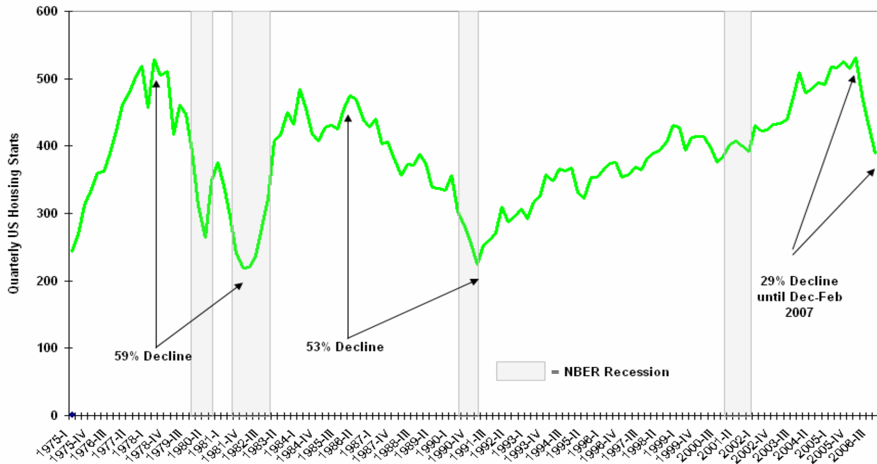
Housing Starts Q1 1975- Q4 2006
